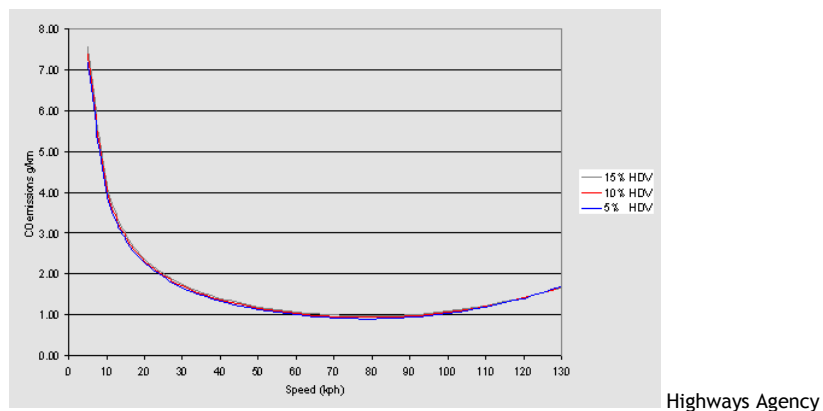
Figure 4: Specific vehicle CO 2 emissions vs. speed
